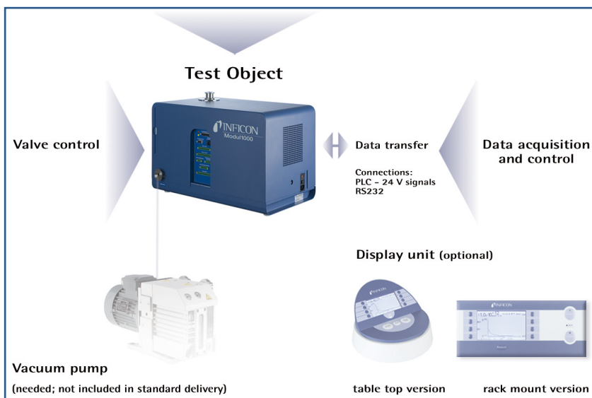
Modul1000 system schematics
