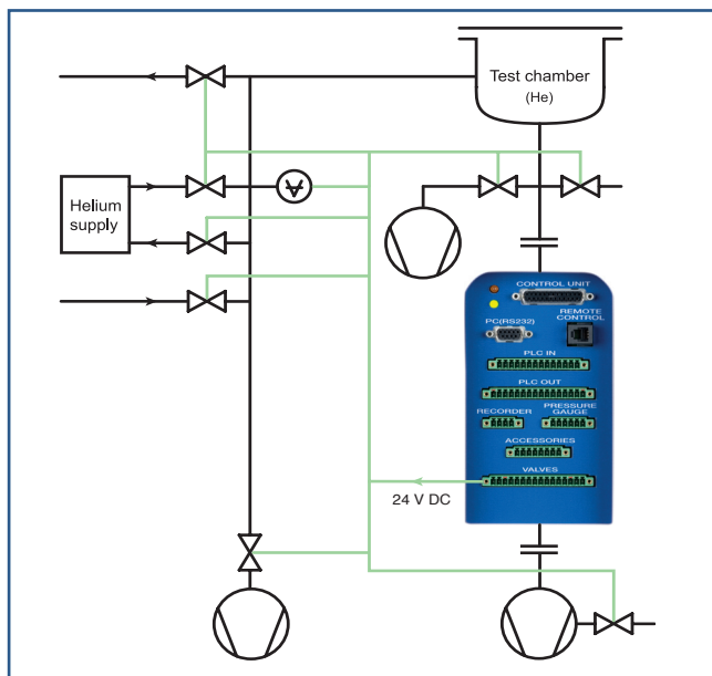
Example: Test station with Helium supply.
